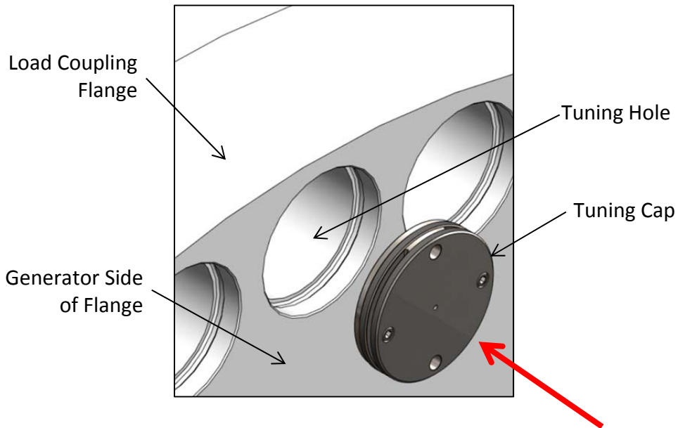
Figure 6A – Inserting Tuning Cap
