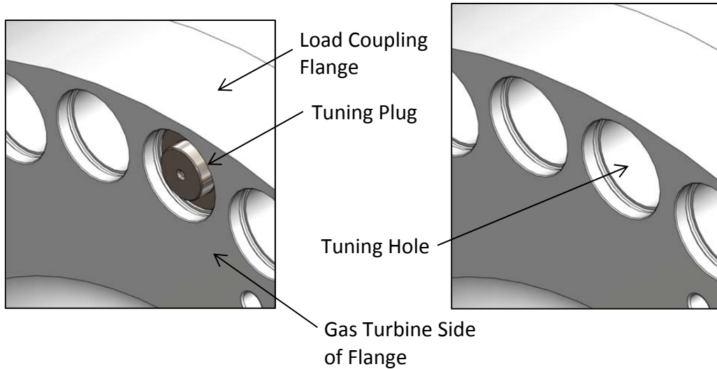
Figure 6F – Inserted Tuning Plug
